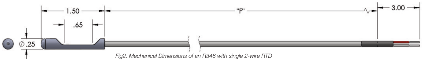
Fig2. Mechanical Dimensions of an R346 with single 2-wire RTD
