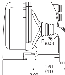
20-pin, Multi-Connector
