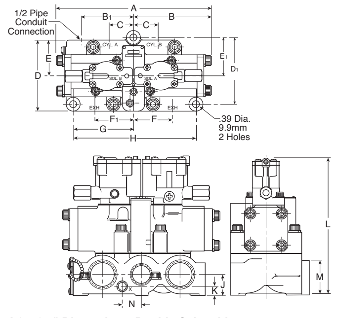
L6558 1" Dimensions, Double Solenoid
