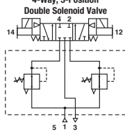
Independent Dual Port Regulator with 4-Way, 3-Position Double Solenoid Valve
