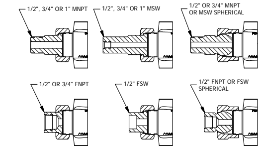
TANK & GAGE CONNECTION (3/4" FSW UNION CONNECTION NOT AVAILABLE AS STANDARD)
